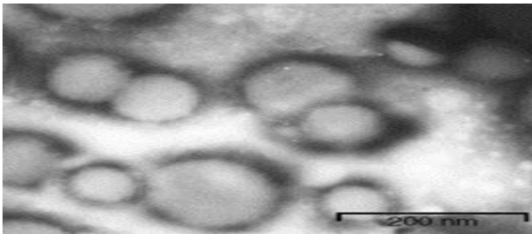
Figure 4: Transmission electron micrograph of optimized BCT-TFS batch M5
