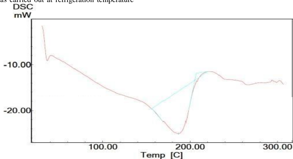
Figure 1: DSC thermogram of Baricitinib
