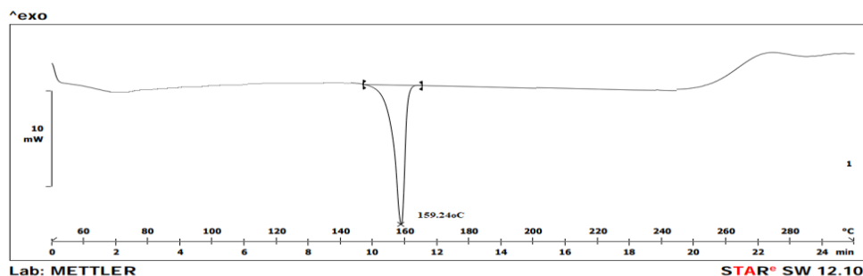
Figure 1: DSC thermogram of Naproxen +Excipients
