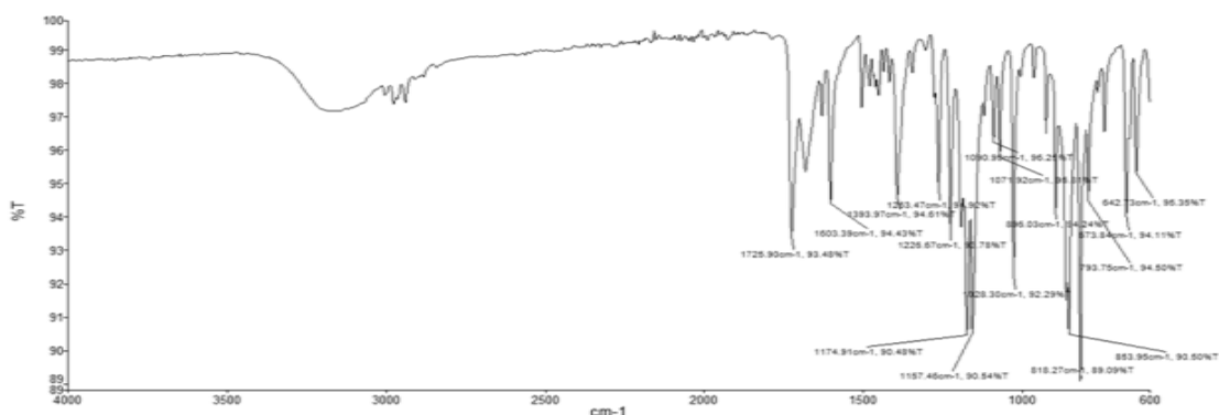
Figure 2: IR spectra of Naproxen
