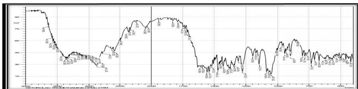
Figure 3: IR spectrum of Ketorolac Tromethamine +HPMC K15M
