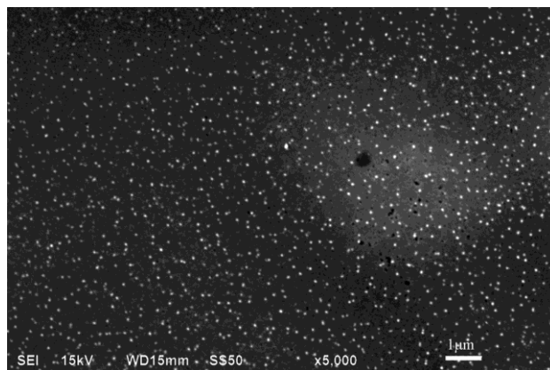
Figure 7 scanning electron micrographs of Lomefloxacin loaded solid lipid nanoparticles consisting of glyceryl monostearate 10%, poloxamer 8%, drug/lipid ratio 13.5% (X5000).
