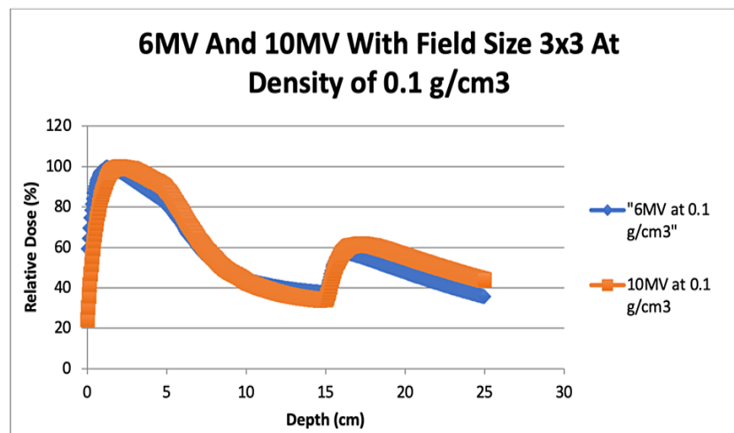
Figure 11: A comparison among the two energies 6MV and 10MV for the same field size 3cm x 3cm and density of 0.1g/cm 3 is made.
