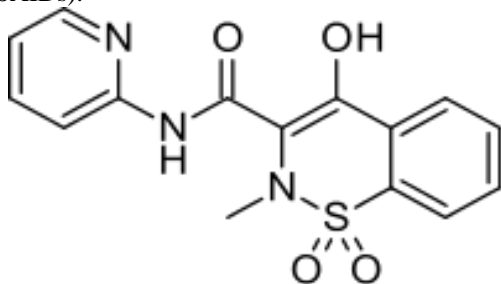
Fig no:1 Structure of piroxicam
